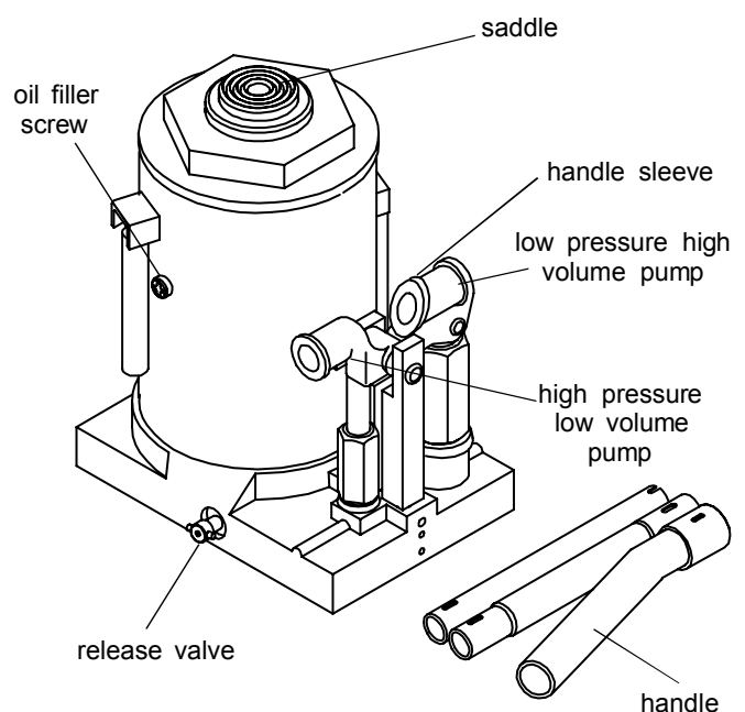
Figure 2 - 10500 Nomenclature
