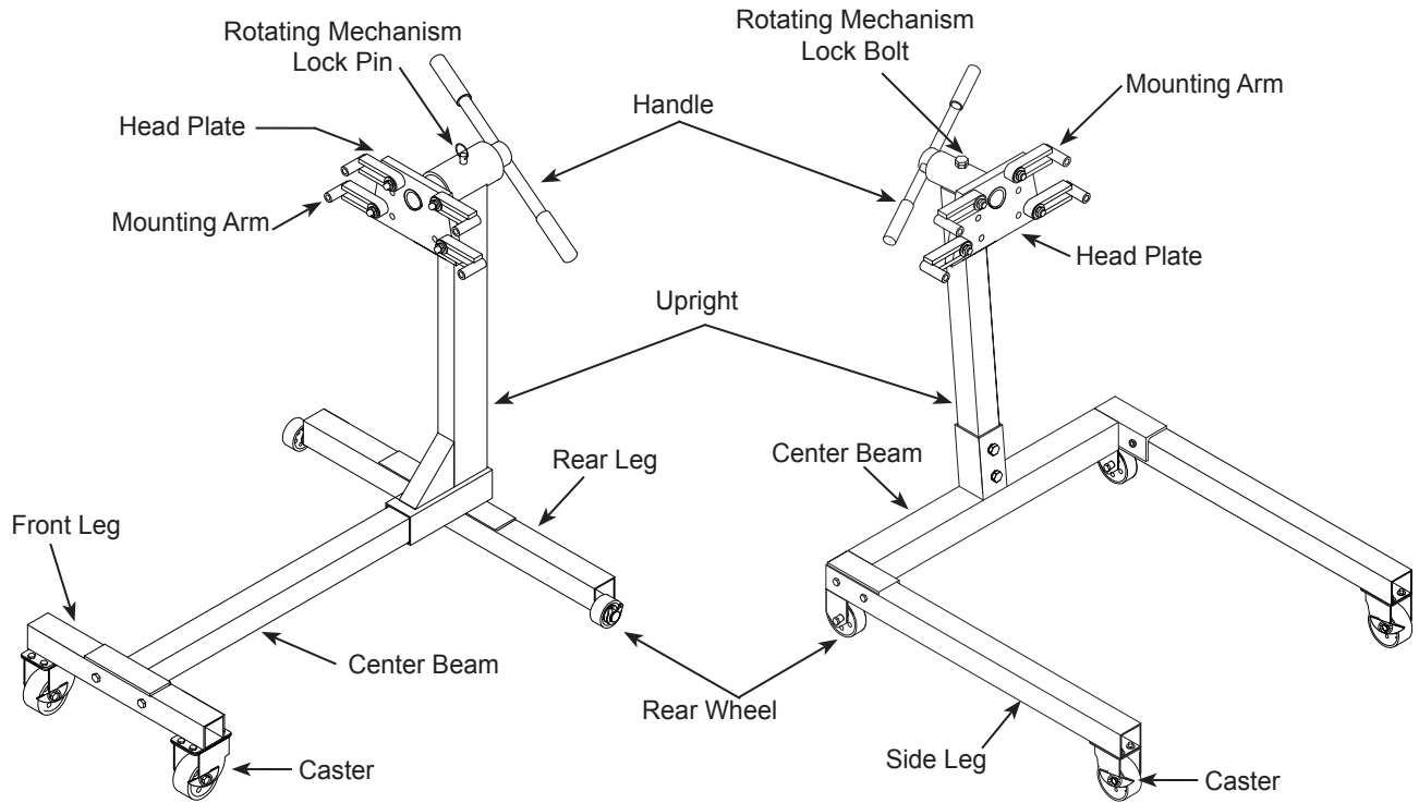
Figure 1 - Model 30750 Components
