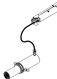
Figure 2 - Pump/ram air bleed
