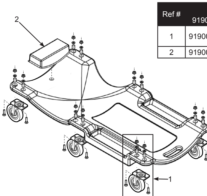
Figure 3 - Creeper Replacement Parts (91901 Shown)
