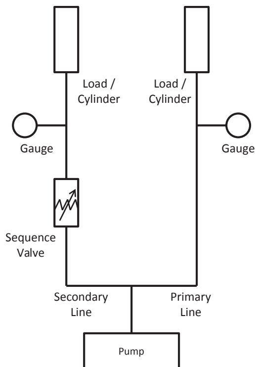
Figure 3 - Typical CVS3 Sequence Valve Connection
