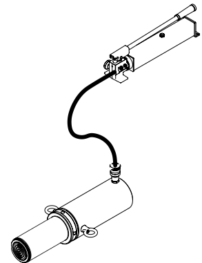
Figure 2 - Illustration to bleed air from system
