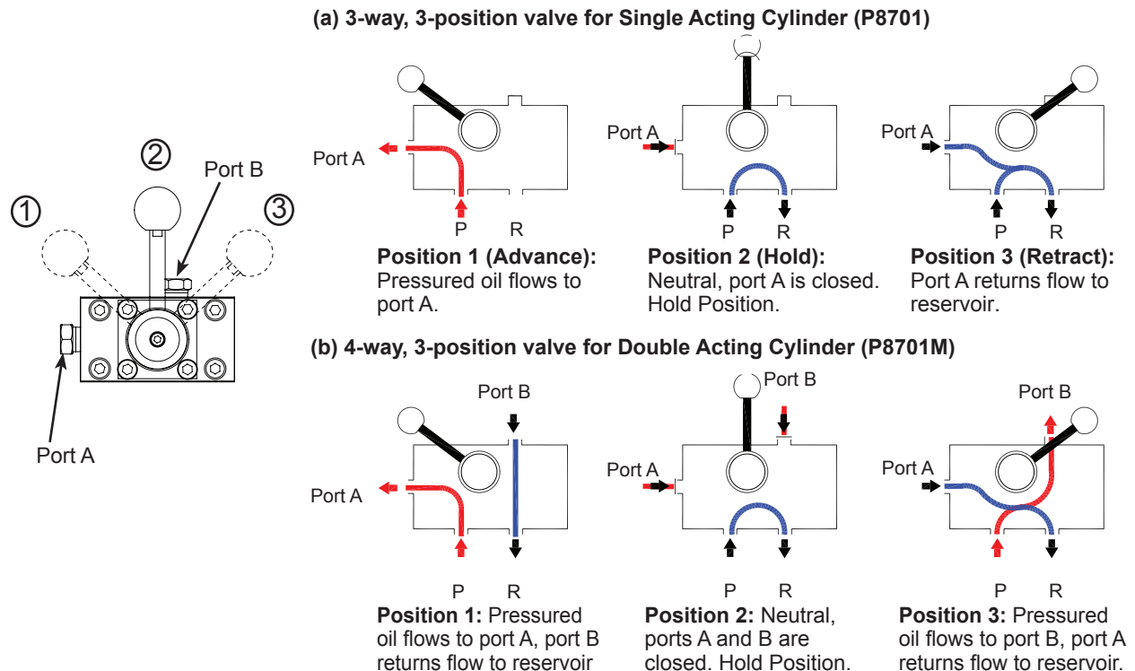
Figure 4 - Flowpath of the valve positions and operations for Model P8701 & P8701M.
